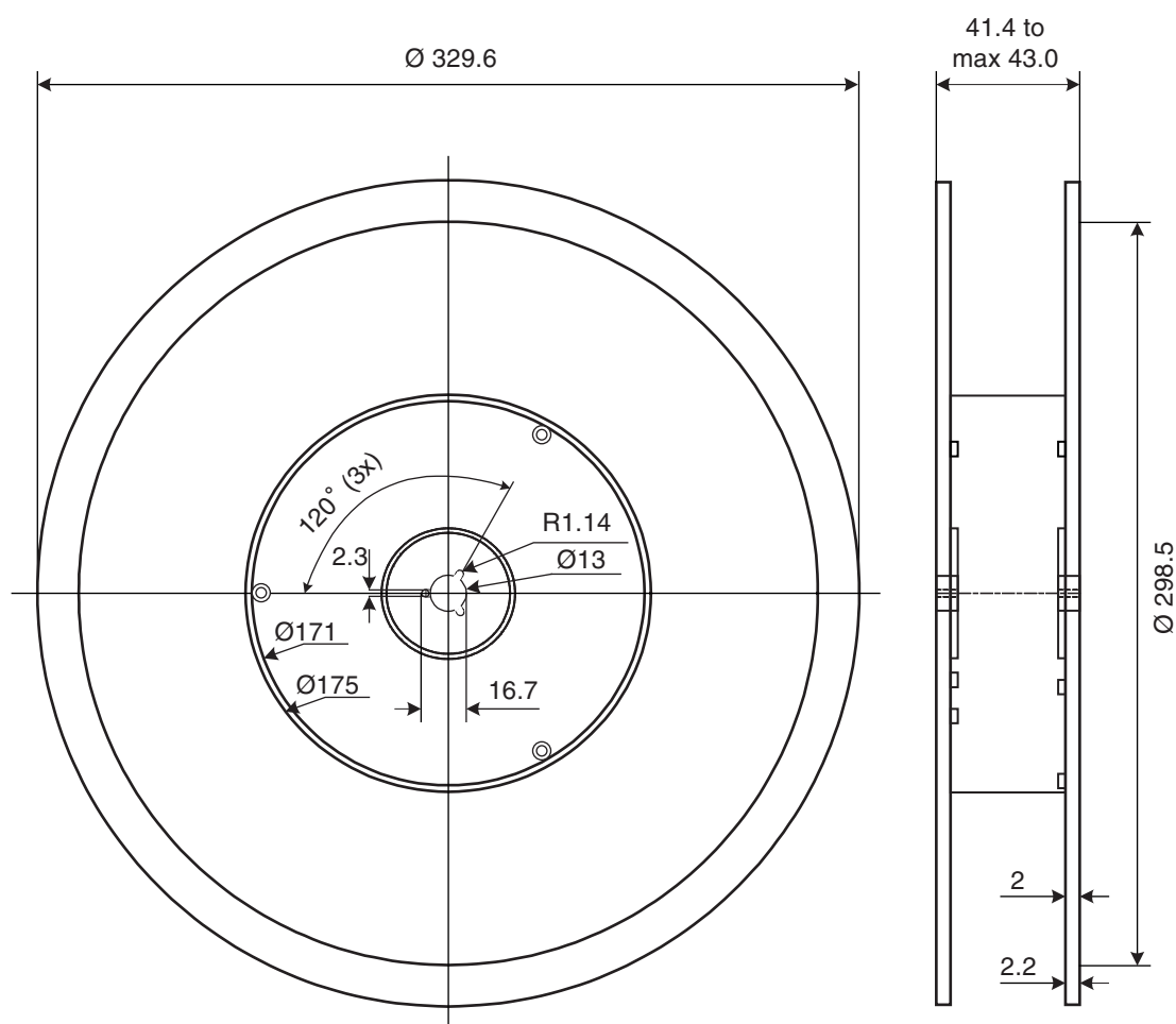
Figure 10-10. Shipping Reel for NOA3 Micromodule
