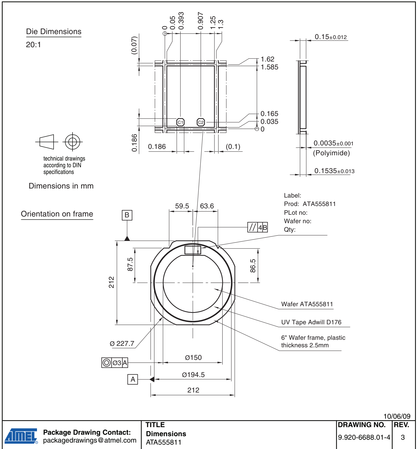
Figure 10-1. 6" Sawn Wafer on Foil with Ring (Type 11, Standard Pads)
