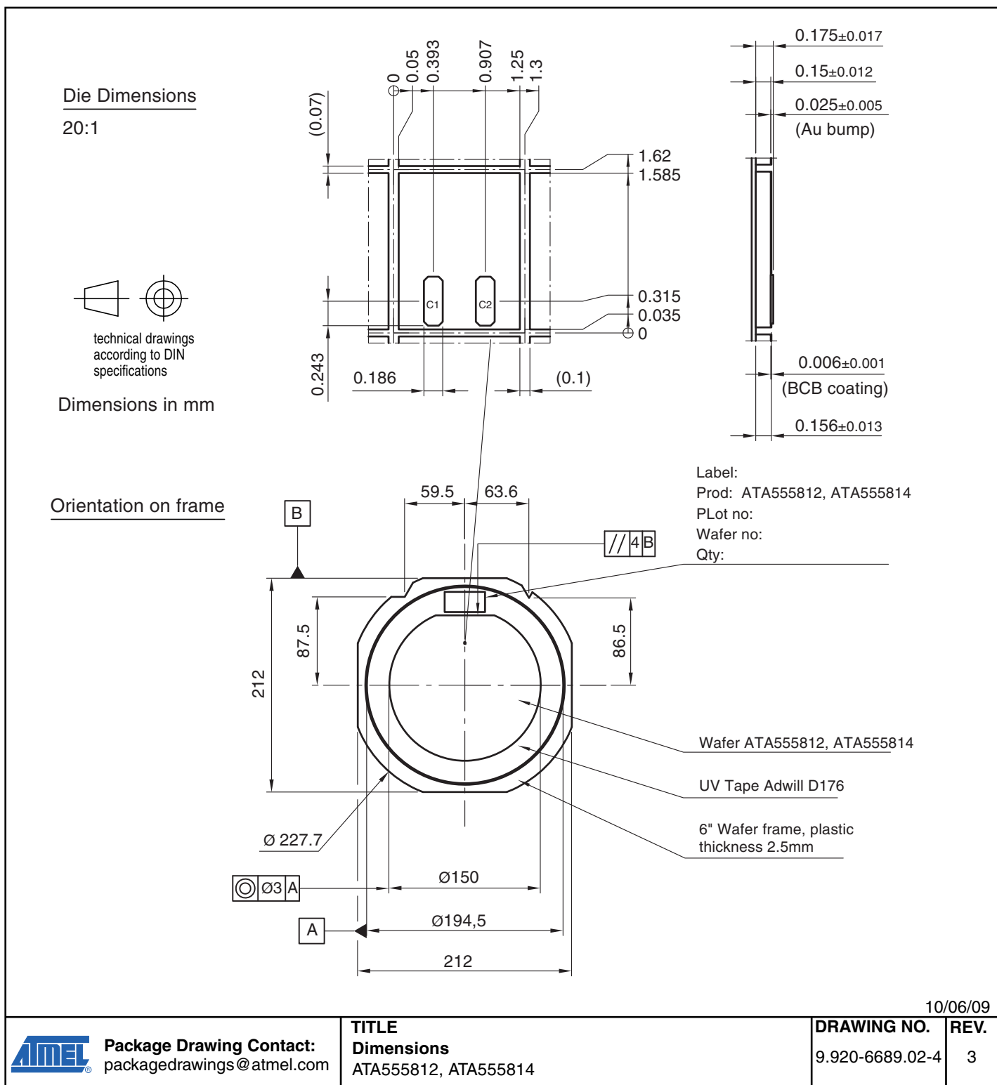
Figure 10-3. 6" Sawn Wafer on Foil with Ring and Goldbumps 25 \mu\text{m} (Type 12/14, Mega Pads)
